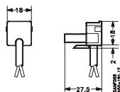
Primary plug
